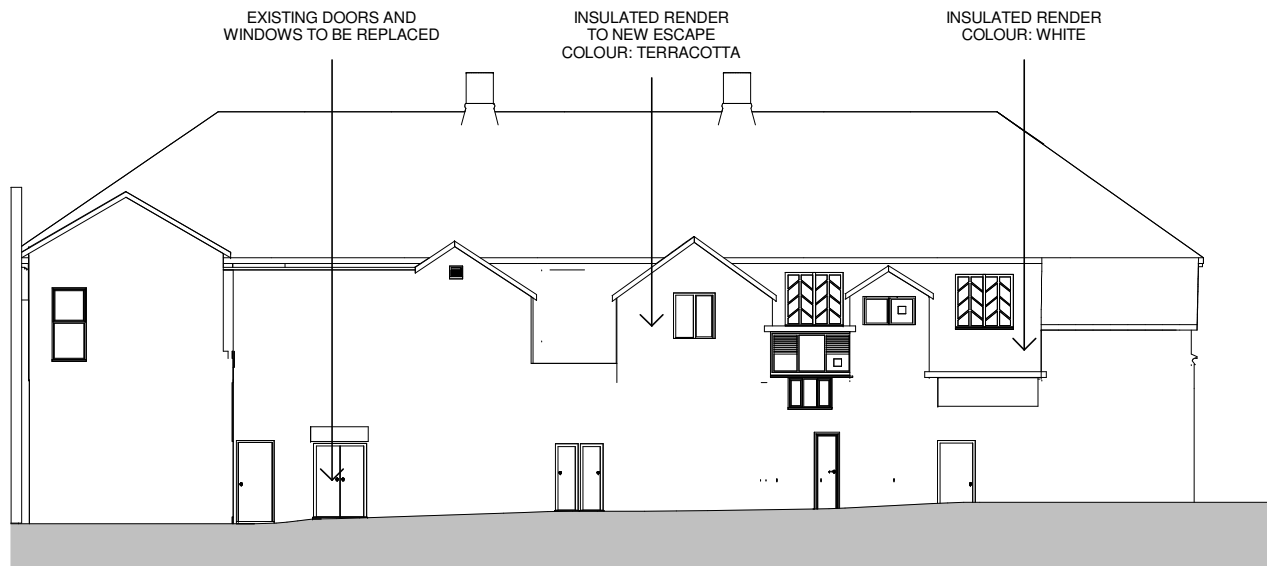
2 PBX_Proposed Elevation CC 1 : 200
